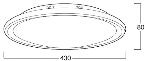
CSP43-021 LED38W 4000K 430 x 430 x 80 mm Price 2,240.-
