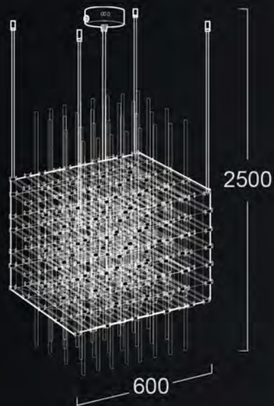
PSG60-250 LED100W 3000K 600 x 600 x 2500 mm Price 22,600.-
